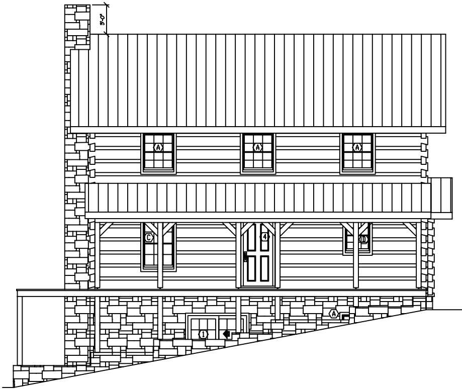
PLAN FRONT ELEVATION
